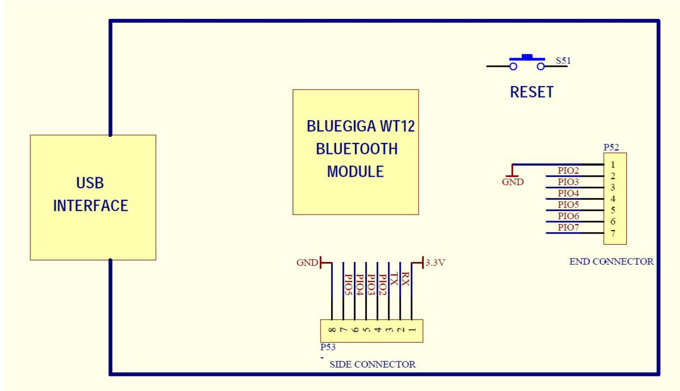
Figure 2 – Expansion Connectors
